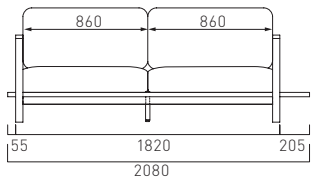
BEBR-SF30(M,A)1R W2080 D935 H788 (SH385)
