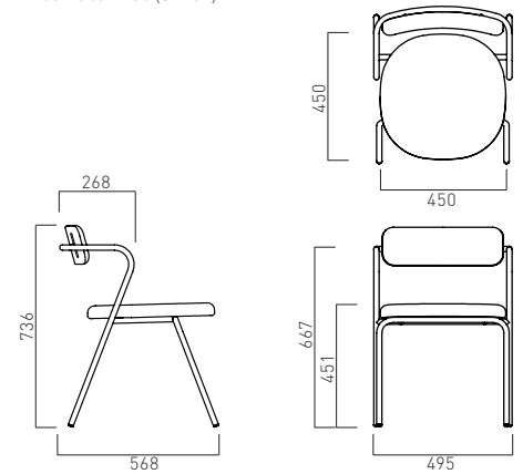
BESI-COA1 W495 D568 H736 (SH451)
