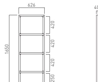
BEBI-1 W626 D40 H1650
