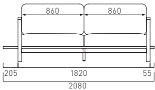
BEBR-SF30(M,A)1L W2080 D935 H788 (SH385)
