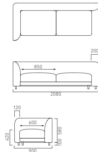
BELO-SFH30L/R W2080 D900 H680 (SH420)
