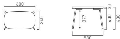
BESP-ST2 W600 D340 H430
