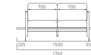
BEBR-SF25(M,A)1L W1760 D935 H788 (SH385)
